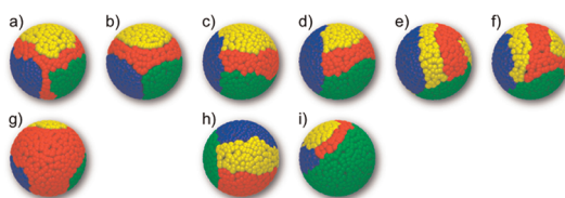
Figure 2. Decorated Cerberus patterns. Tails are not shown. Red: short, blue: medium, green: long, and yellow: longest surfactant. (a) through (f) show different patterns. (a) and (g) and also (d) and (i) show the same type of pattern but obtained with different stoichiometric compositions. (c) and (h) also show the same pattern, but with different chemical ordering due to different combinations of surfactant lengths.
